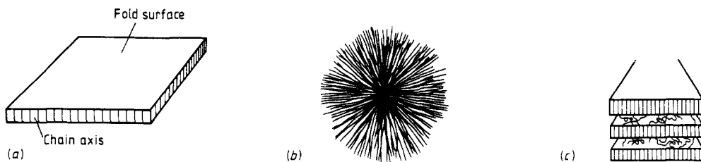
Figure 1. (a) Polymer single crystal lamella. (b) Spherulite consisting of chain folded lamellae radiating from a central point. (c) Magnified end-on view of spherulite, showing stacks of lamellae and interlamellar links. The radial distance R is so large that L is virtually independent of R .
